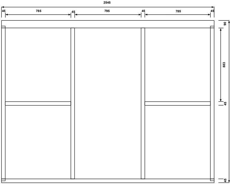
FRONT WALL
